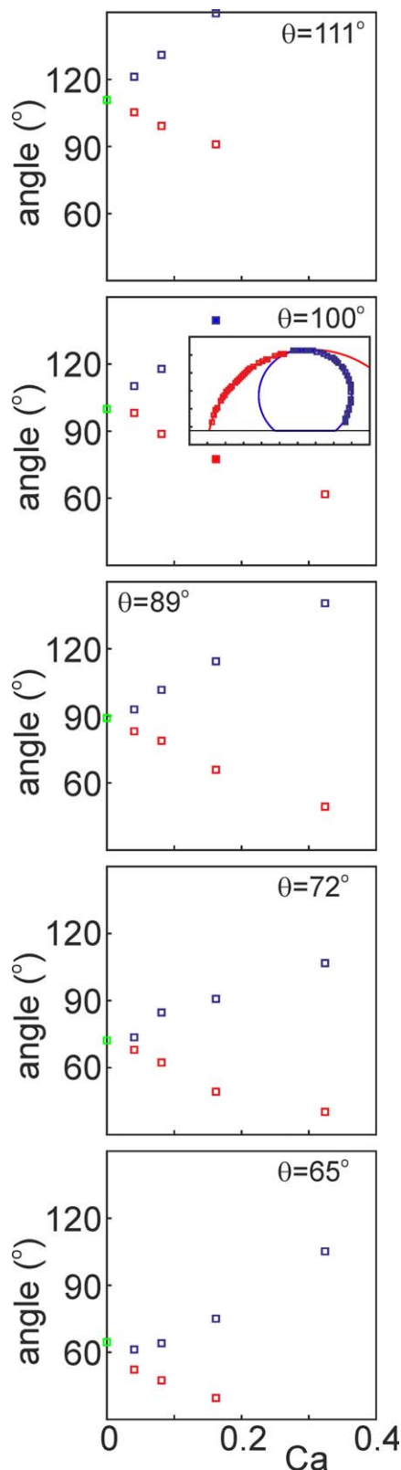
Figure 12. Receding contact angle \theta_r (red symbols) and advancing angle \theta_a (blue symbols) as a function of Ca for all static contact angles \theta (green symbols) investigated.
