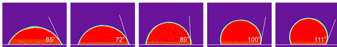
Figure 5. Equilibrated droplet shapes and contact angle estimates.
