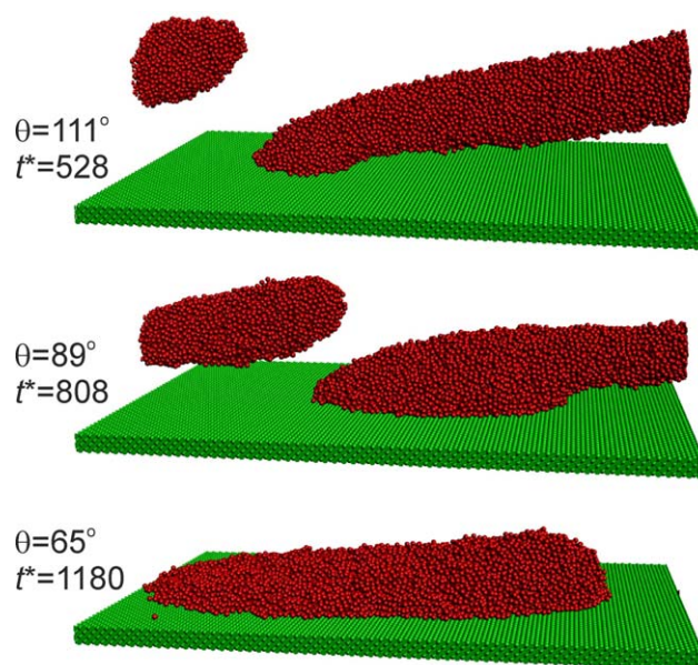
Figure 13. Impressions of drop deformation at Ca = 0.64 for three static contact angles.
