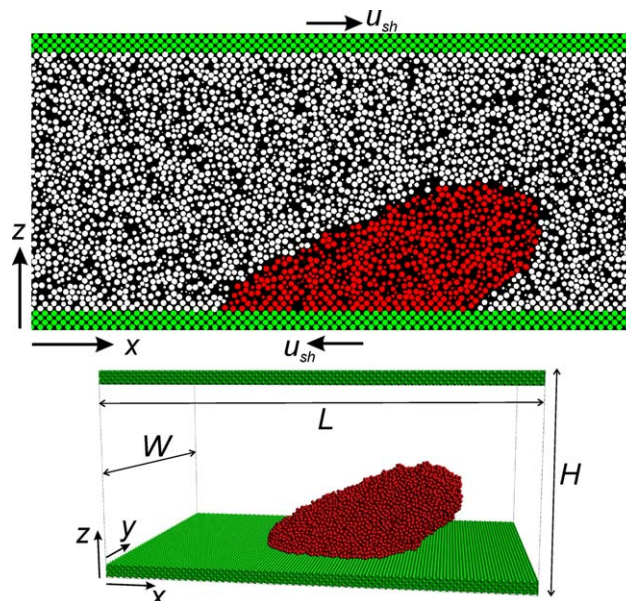
Figure 1. Simulation domain and coordinate system.
