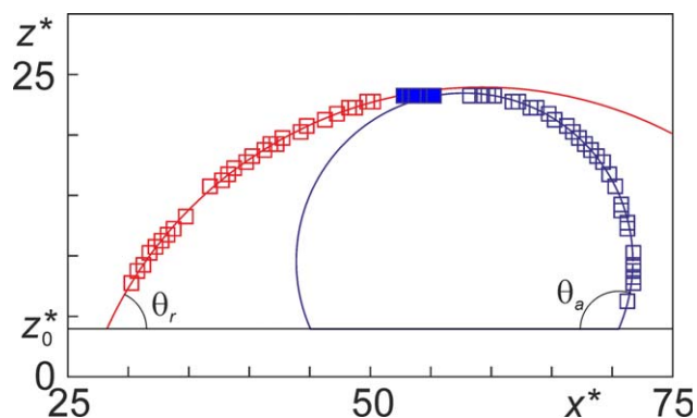
Figure 11. Fitting procedure for determining the receding and advancing contact angles ( \theta_r and \theta_a , respectively).
