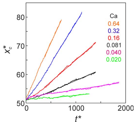
Figure 7. Footprint center position ( x_c^* ) as a function of time for various capillary numbers.
