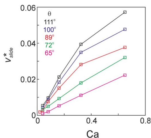
Figure 8. Steady-state droplet sliding velocity as a function of the capillary number for droplets that have static contact angle \theta as indicated.
