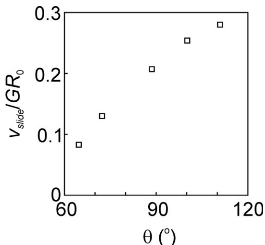
Figure 9. Sliding velocity relative to shear rate times initial drop radius as a function of the static contact angle \theta .
