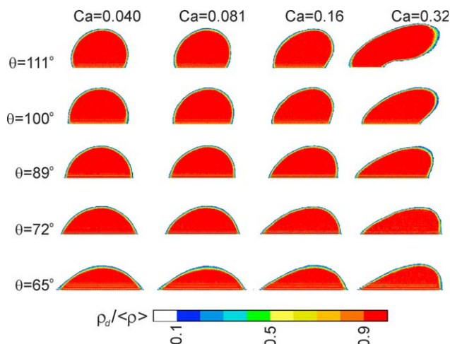
Figure 10. Time-averaged shape of sliding droplets.
