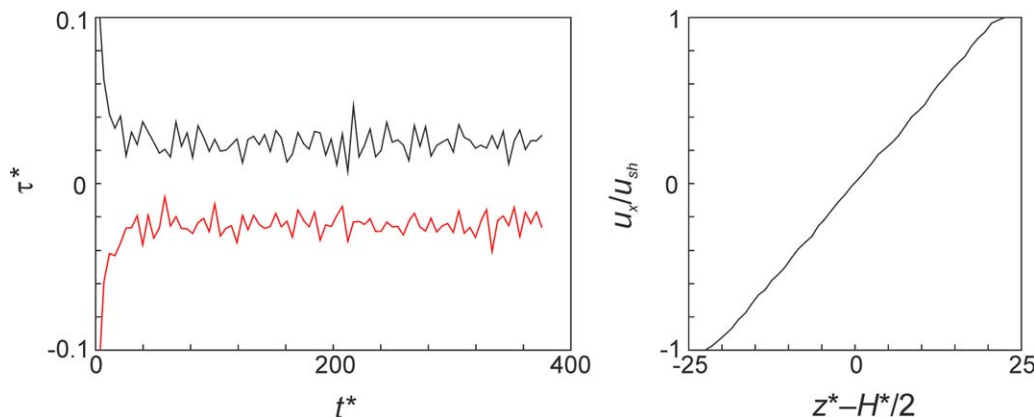
Figure 2. Left: Time series of the shear stress \tau^* \equiv \tau \sigma^3 / \varepsilon on the top (black) and bottom (red) solid wall in a single-phase shear simulation; each data point is the average of 1000 time steps with \Delta t^* = 0.0046 . Right: Average wall-normal x-velocity profile. In this case, u_{sh}^* \equiv u_{sh} \sqrt{m/\varepsilon} = 0.14 .
