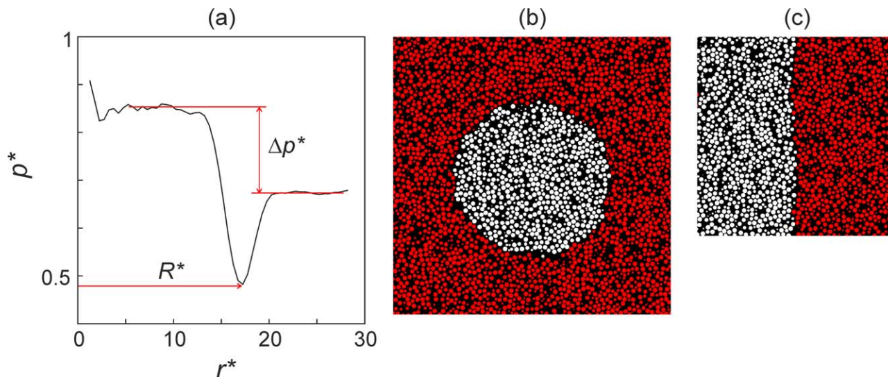
Figure 4. Determining surface tension. (a) Radial pressure profile (with resolution \Delta r^* = 2.5 ) inside and outside the drop a cross section of which is shown in (b). (c) Cross section through the simulation domain for determining surface tension of a planar interface via the virial route.
